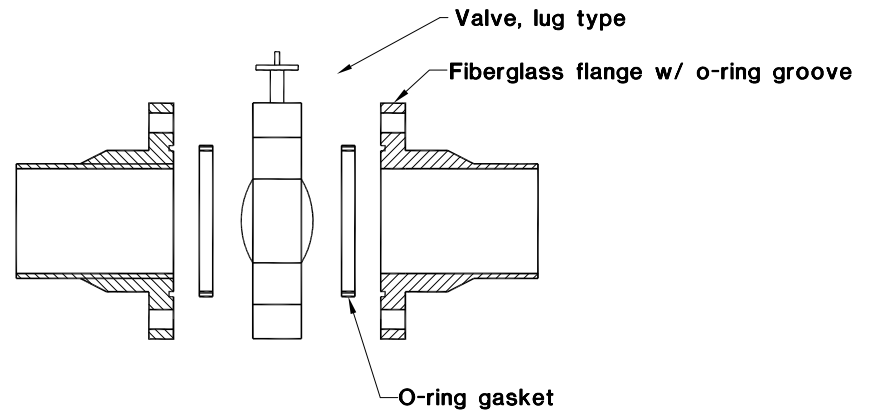
Fiberglass to full-face or lug type valve flanged joint (with o-ring gasket)
