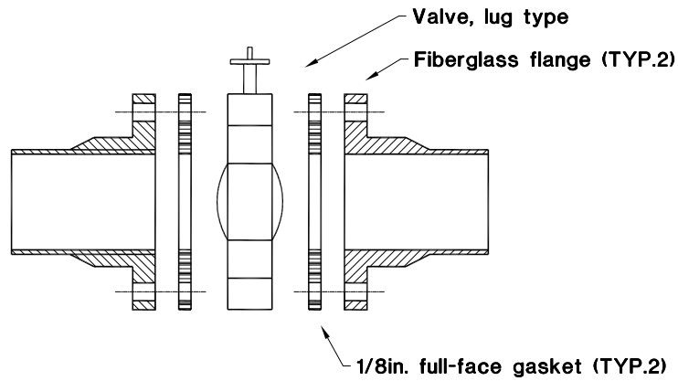
Fiberglass to full-face or lug type valve flanged joint (with full-face gasket)
